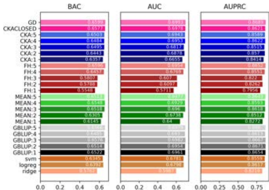
Fig. 2 Figure showing the balanced accuracy (BAC), area under the ROC curve (AUC), and area under the precision-recall curve (AUPRC) for the benchmark of our GMKL approaches with GBLUP and other ML methods on the IBDSNP dataset
