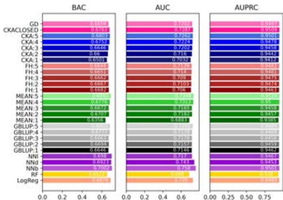
Fig. 3 Figure showing the comparison between the nine methods we benchmarked on the IBDWES dataset. The MEAN, FH, and CKA GMKL approaches using one to five kernel matrices are respectively shown in shades of green, red, and blue. The black to gray bars show the additive GBLUP models, while the bottom bars show the performance obtained by the Neural Networks methods proposed in [50]
